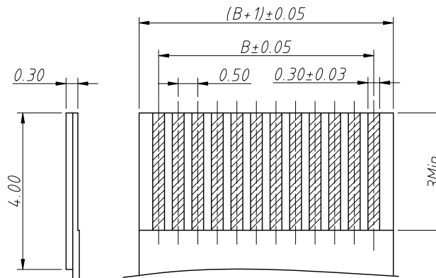
Applicable FPC
