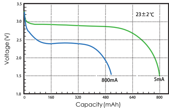
1. Typical discharge profiles at 23±2°C (at mid-discharge)
