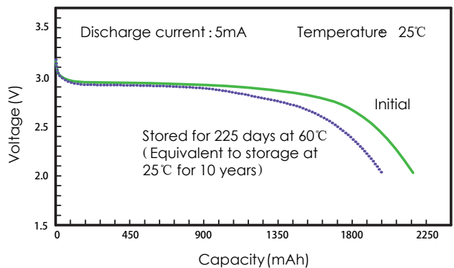
3. Storage characteristics
