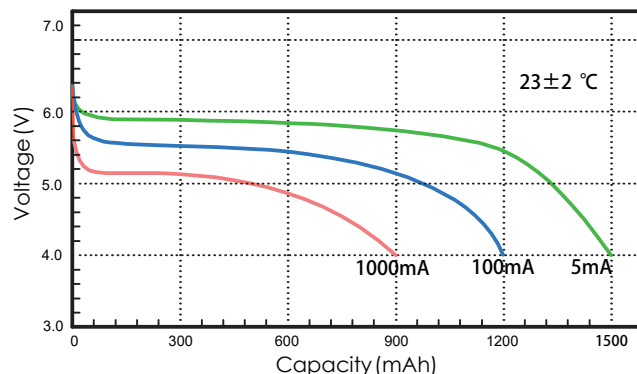
1. Typical discharge profiles at 25°C (at mid-discharge)
