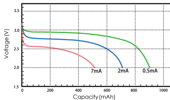
1. Typical discharge profiles at 25°C (at mid-discharge)
