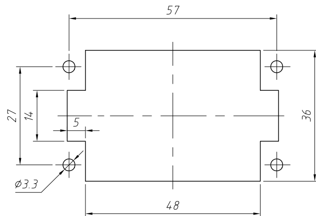
Panel Cut
