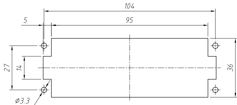
Panel Cut
