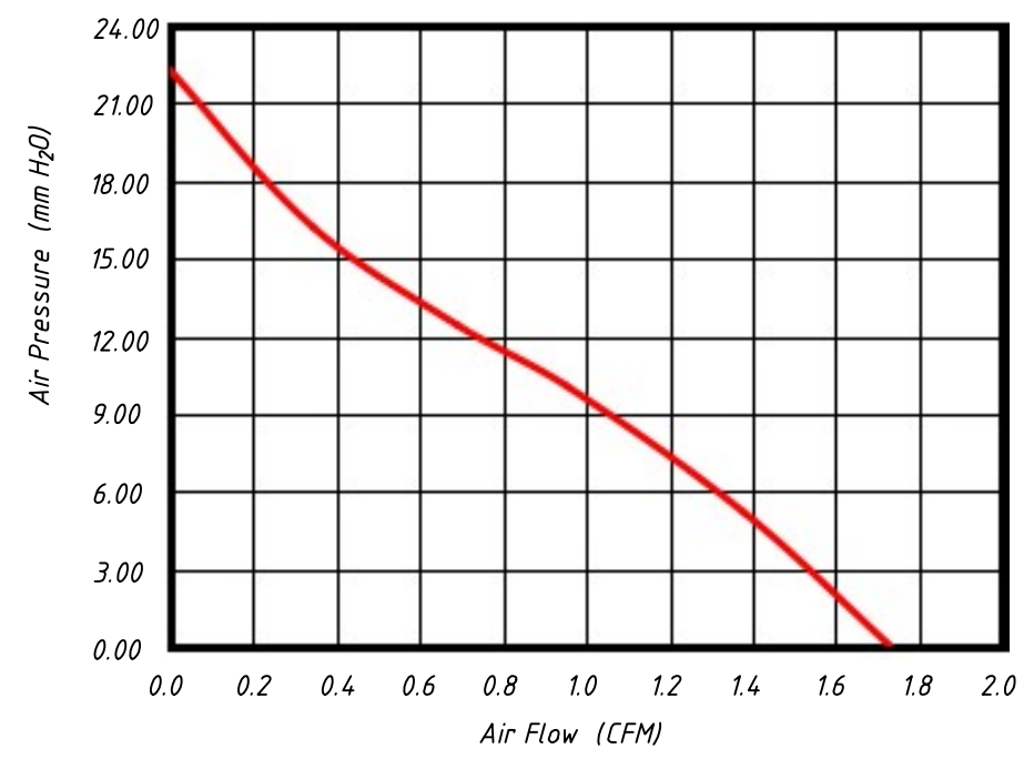
P&Q Curve (Under Rated Voltage)
