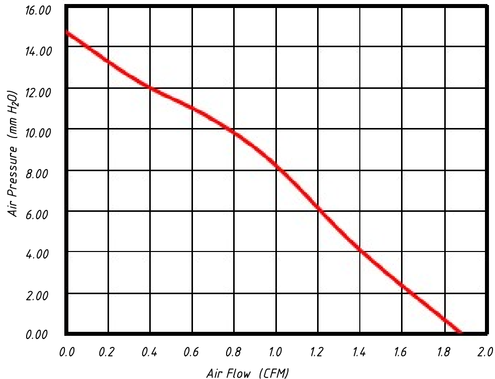
P&Q Curve (Under Rated Voltage)
