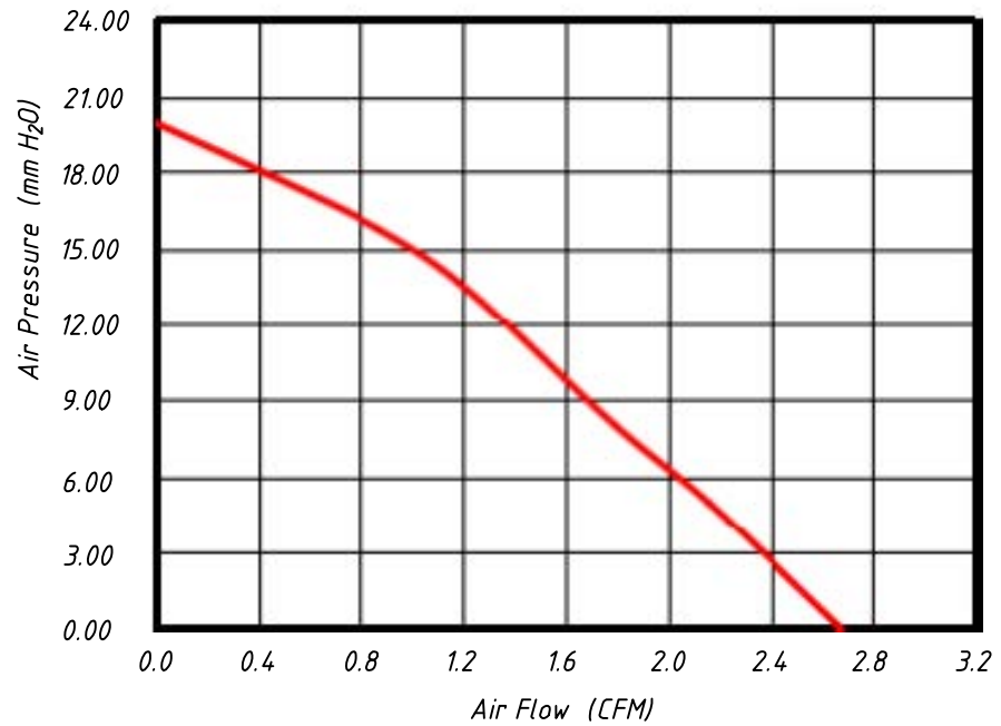
P&Q Curve (Under Rated Voltage)
