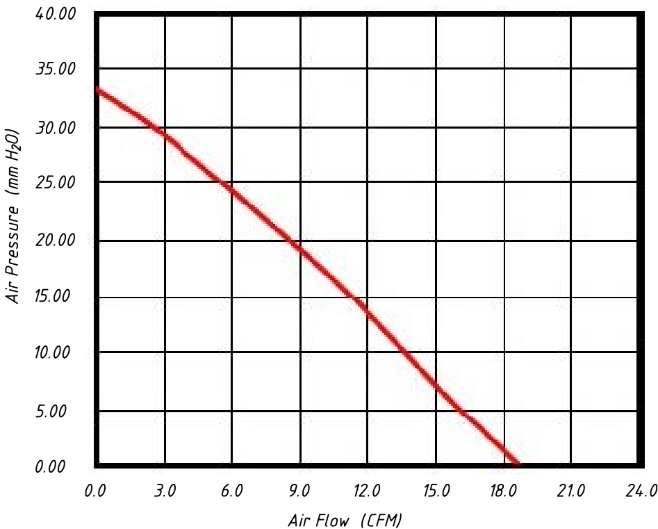
P&Q Curve (Under Rated Voltage)
