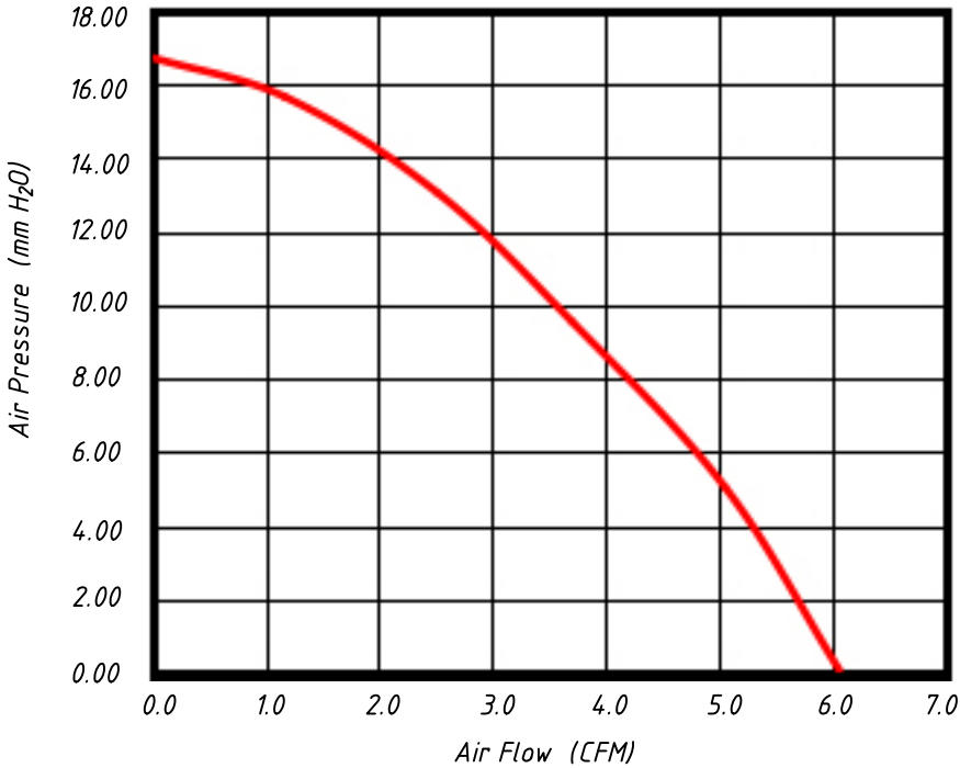
P&Q Curve (Under Rated Voltage)
