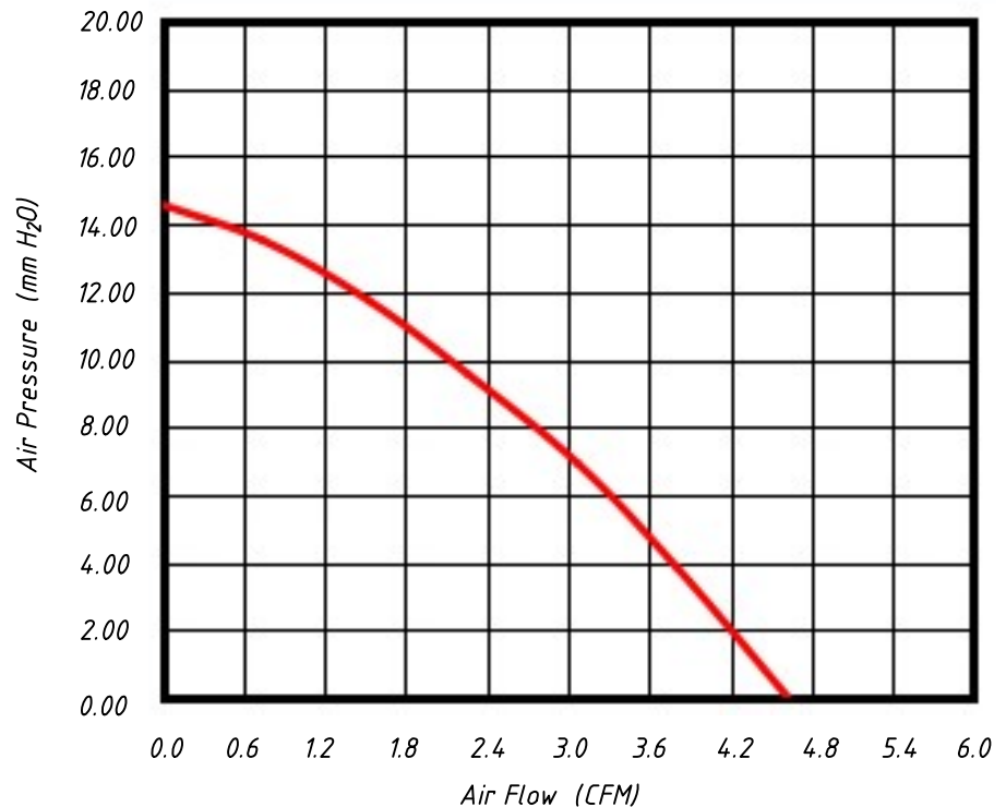
P&Q Curve (Under Rated Voltage)
