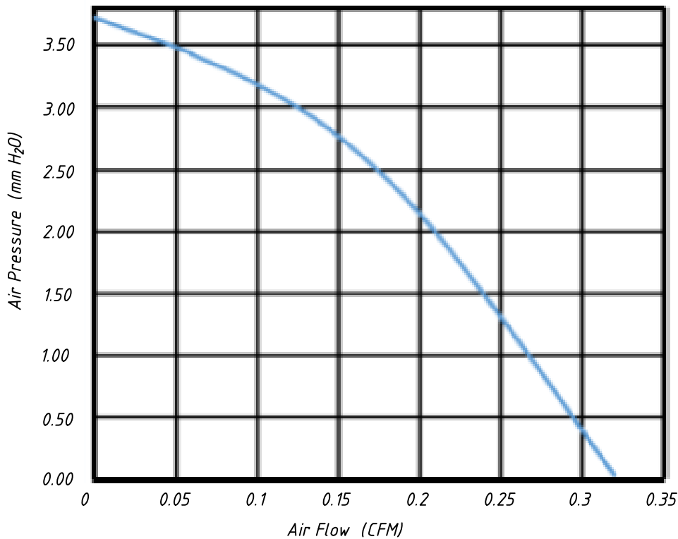
P&Q Curve (Under Rated Voltage)
