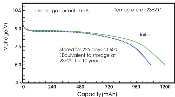
3. Storage characteristics
