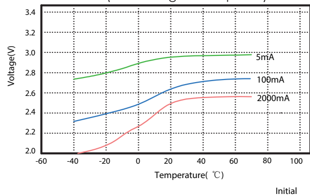
2. Voltage plateau versus Current and Temperature (at discharge stable phase)
