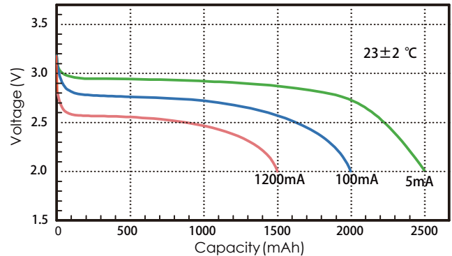
1. Typical discharge profiles at 25°C (at mid-discharge)
