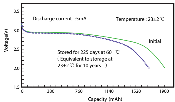
3. Storage characteristics
