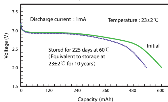
3. Storage characteristics
