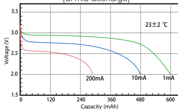
1. Typical discharge profiles at 23\pm 2^\circ\text{C} (at mid-discharge)
