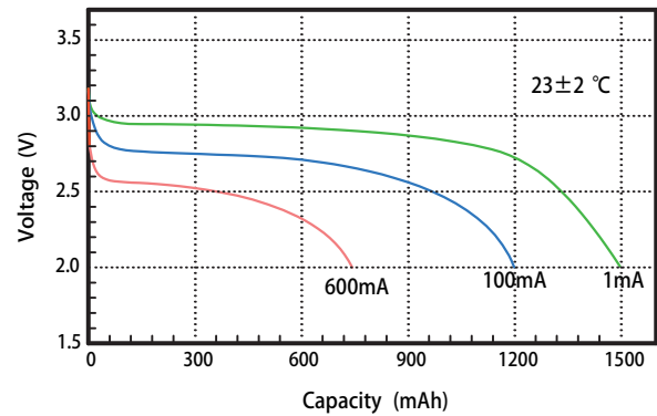
1. Typical discharge profiles at 25°C (at mid-discharge)
