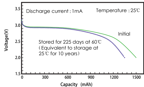
3. Storage characteristics
