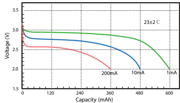
1. Typical discharge profiles at 23\pm2^\circ\text{C} (at mid-discharge)
