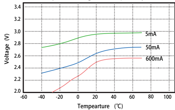
2. Typical discharge profiles with different current (at discharge stable phase)
