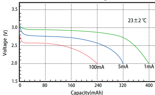
1. Typical discharge profiles at 23±2°C (at mid-discharge)
