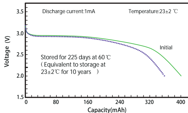
3. Storage characteristics
