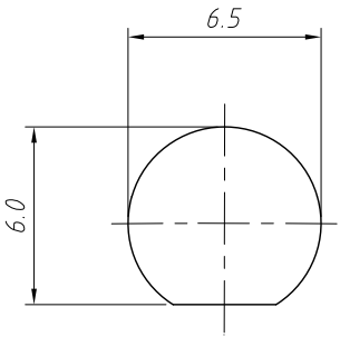
Recommended Mounting Hole Dim's
