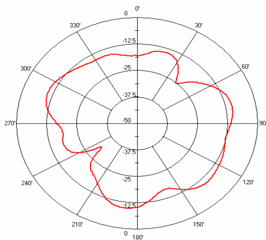
2.45 GHz E-Plane vertical
