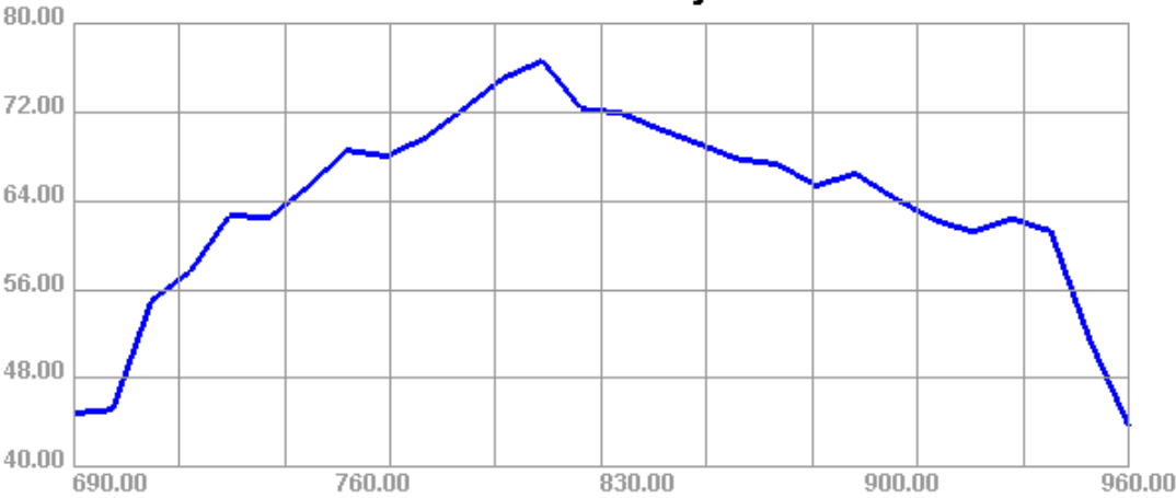
690.00MHz - 960.00MHz Efficiency
