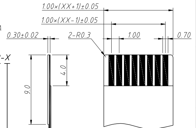
Accommodated FFC (Scale 2:1)
