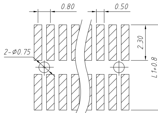
Recommended P.C.B Hole Layout
