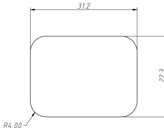
PANEL CUT-OUT
