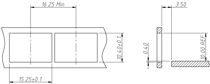
Bezel Recommended Bezel Thickness: 0.80 ~ 2.60mm Bezel Opening Below Top Of PCB
