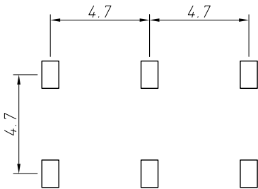
Recommanded PCB Layout
