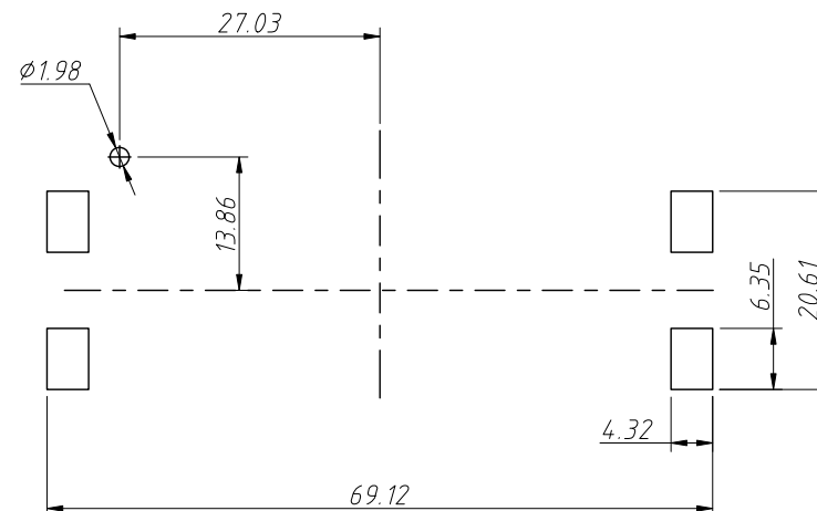
PCB Layout
