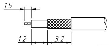
Cable stripping size
