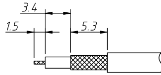
Cable Stripping Size
