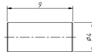
Copper Tube
