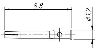
Pin Contact
