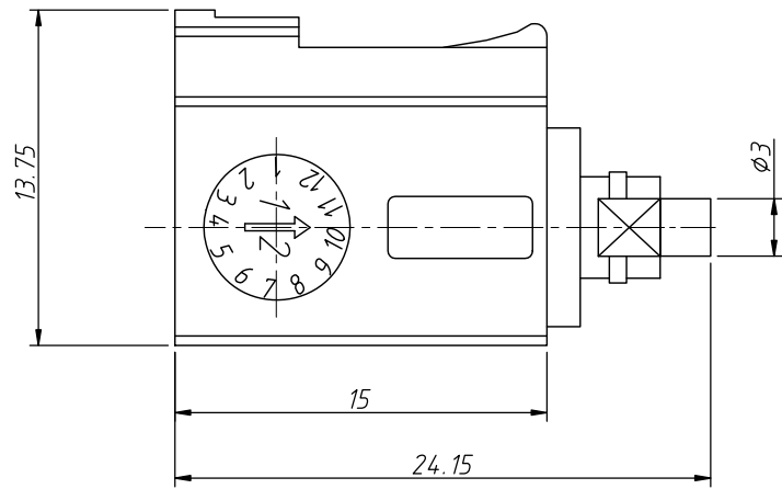
Plastic Housing
