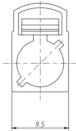
FAKRA C Jack
