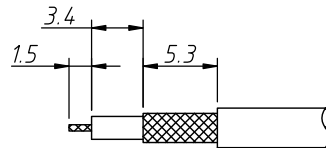
Cable Stripping Size
