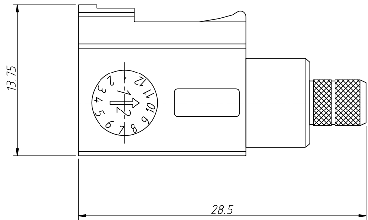
Plastic Housing
