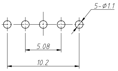
Mounting
