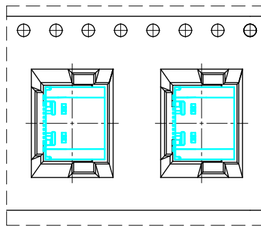
DETAIL X
