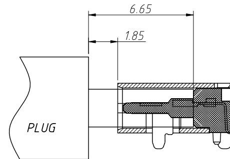
AFTER MATING
