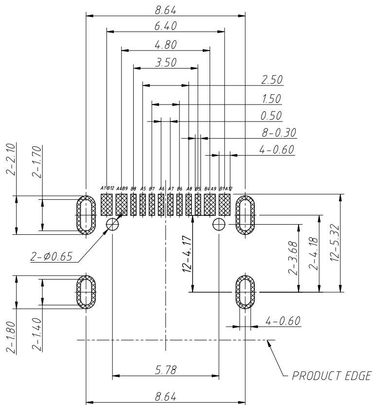
Recommended PCB Layout Tolerance: ±0.05mm, T=0.80
