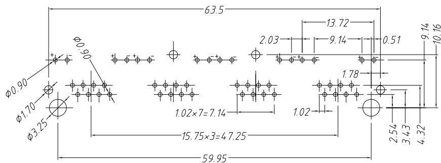
PCB Layout
