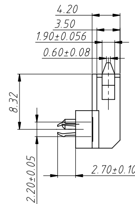
Section B-B
