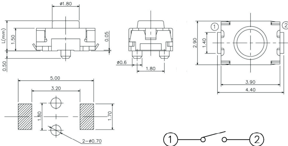
Mounting Holes
