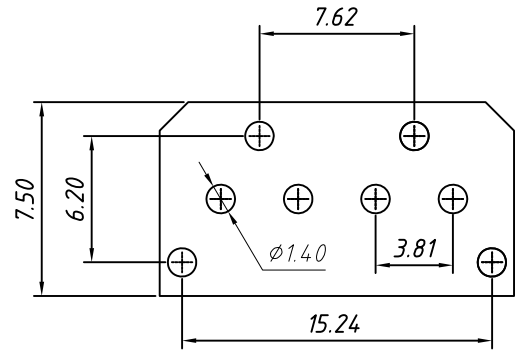
PCB LAYOUT Tol: ±0.05mm
