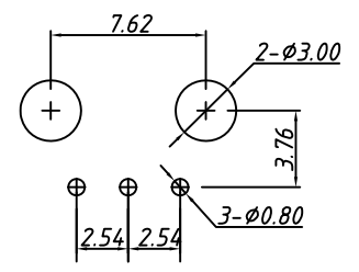
P.C.B LAYOUT TOLERANCE:±0.30
