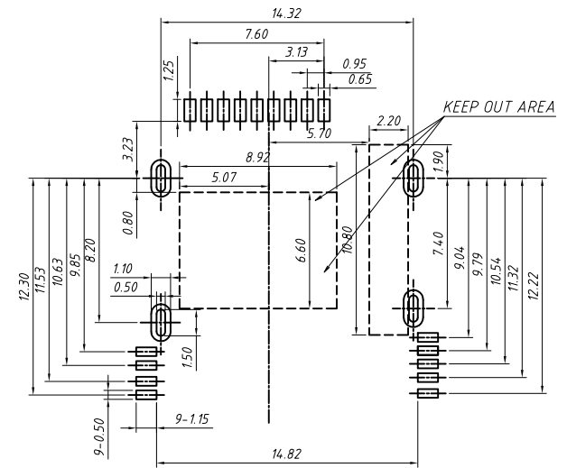
RECOMMENDED PCB LAYOUT TOLERANCE UNLESS OTHERWISE IS \pm 0.05
