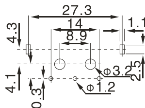
C=14:PCB LAYOUT
