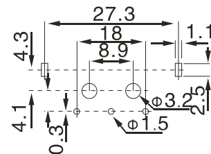
C=14:PCB LAYOUT
