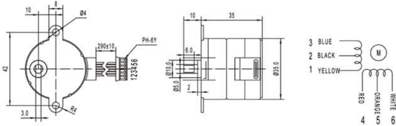
Gear Motor Dimensions (mm)
