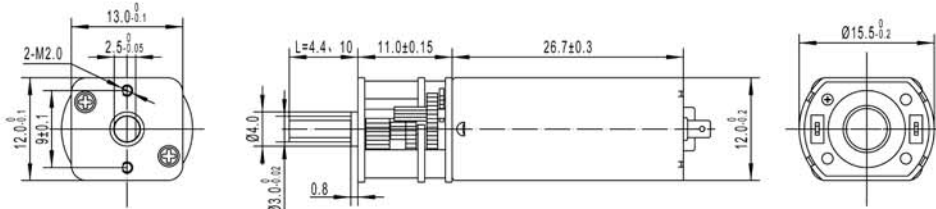
Gear Motor Dimensions (mm)
