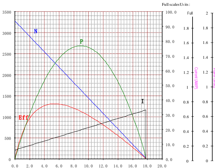
Performance Curve : B3020FB-S01
