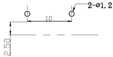
Mounting hole details
