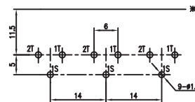
T:1.6 Dimensions of PC board holes Tolerance : ±0.1(Printed-top view)
