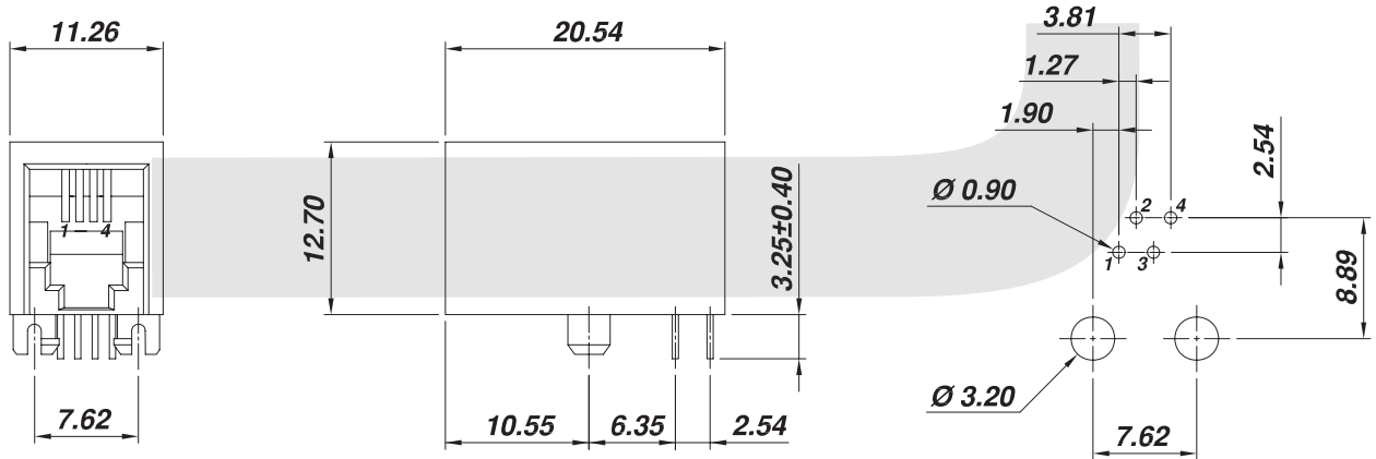
PCB LAYOUT (Top View)
